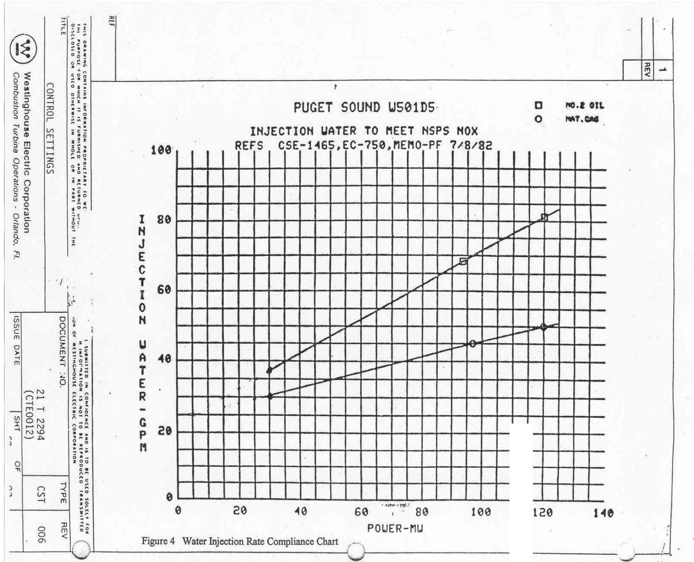
Westinghouse Chart 21 T 2294 – Water Injection Curves for NO x Control · Units 1 and 2
