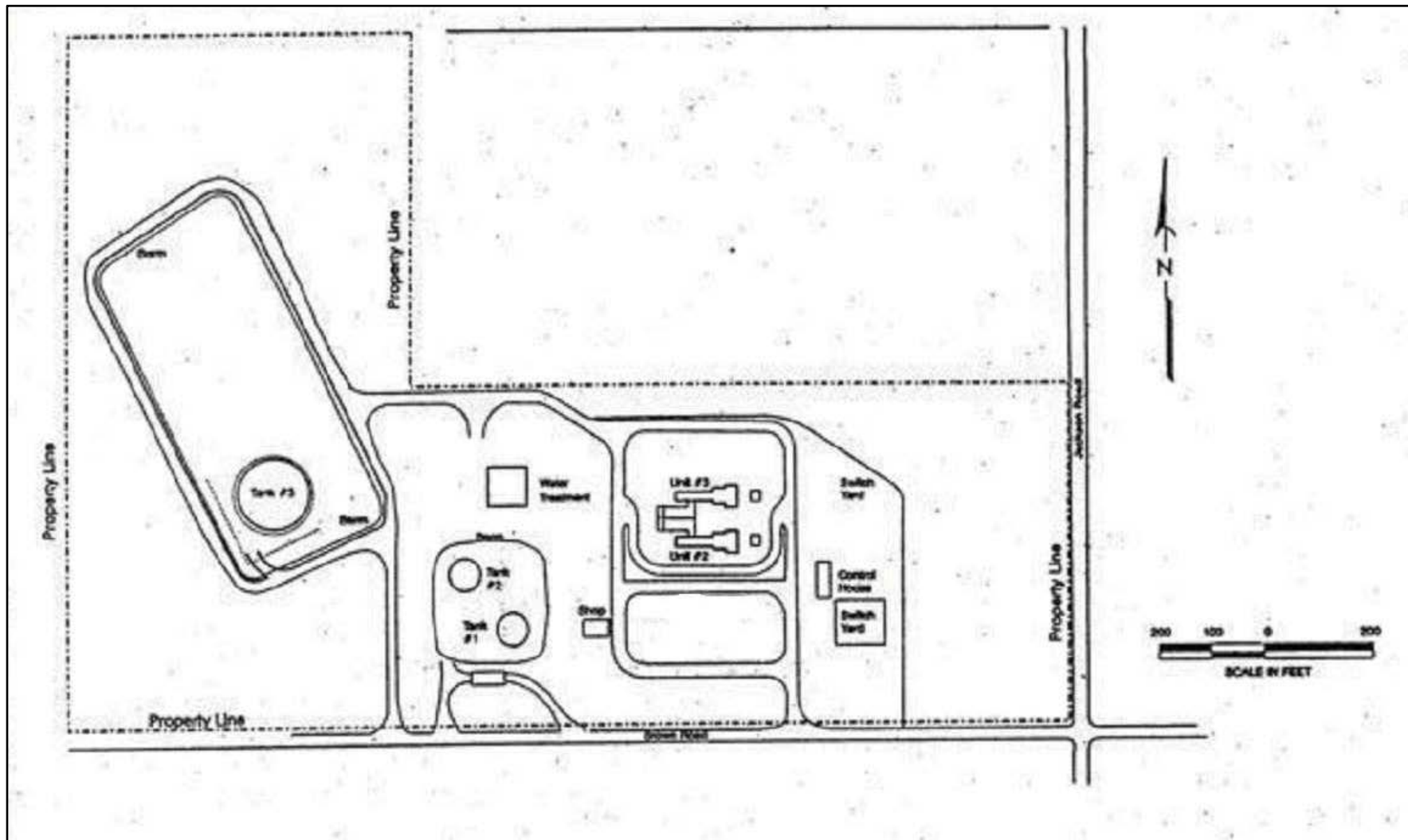
Figure 2 PSE Whitehorn Site Plan
