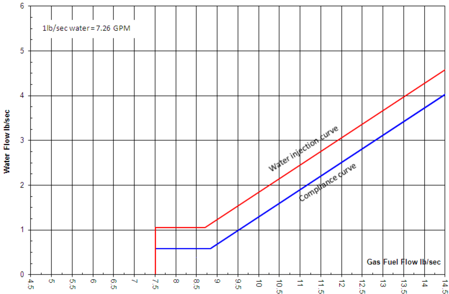
General Electric Water-to-Fuel Injection Compliance Curves – Natural Gas
