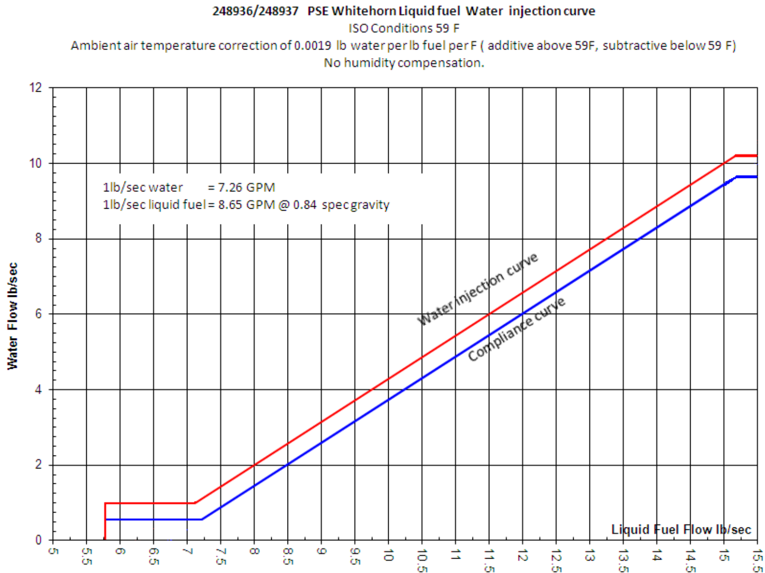
General Electric Water-to-Fuel Injection Compliance Curves – Distillate Fuel
